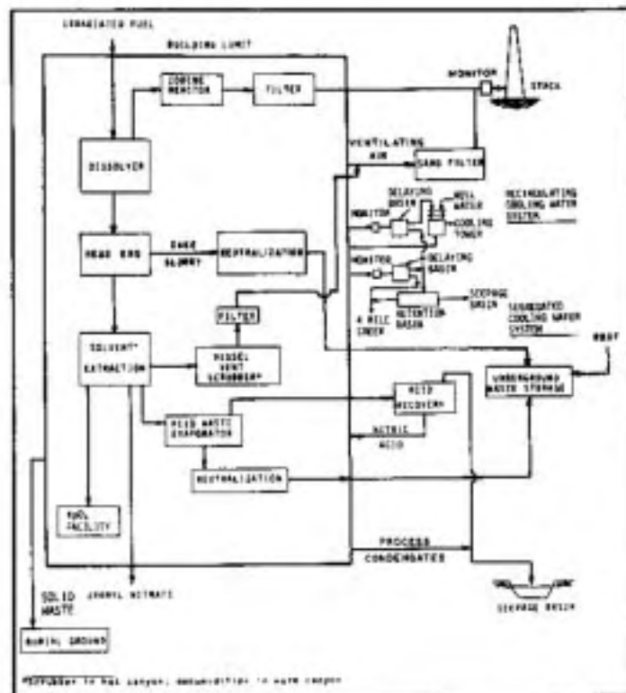
Figure 77 H-Area Separations Diagram
