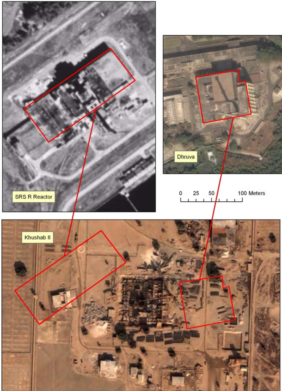
Images of the Khushab II, DHRUVA and R-Reacto, reproduced at the same scale.
