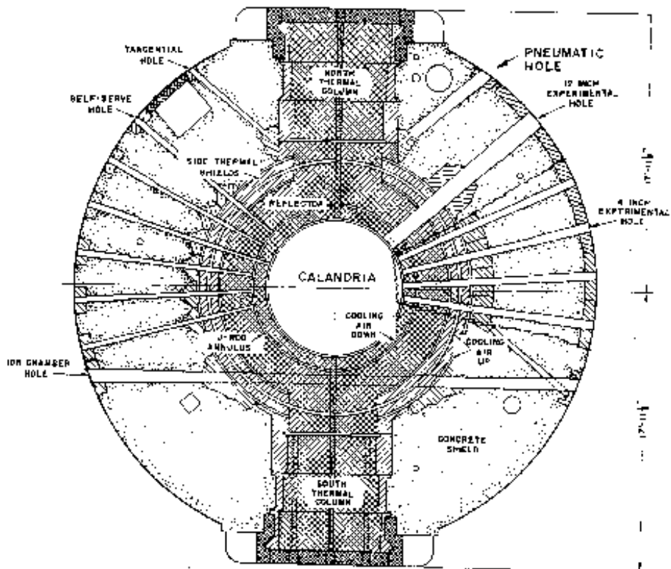
Figure 7-1 Plan Cross Section Through the Reactor Structure
